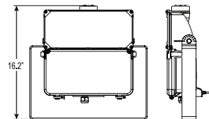
Yoke Mount: EPA of 1.22 Ft 2 and max weight 20 lbs.
