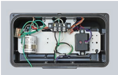
Removable electrical tray with MOV pack surge protection, optional 3-position terminal block and adjustable output module
