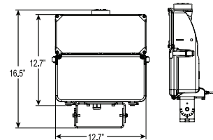
Trunnion Mount: EPA of 1.22 Ft 2 and max weight 18 lbs.
