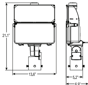
Tenon Mount: EPA of 1.32 Ft 2 and max weight 19 lbs.
